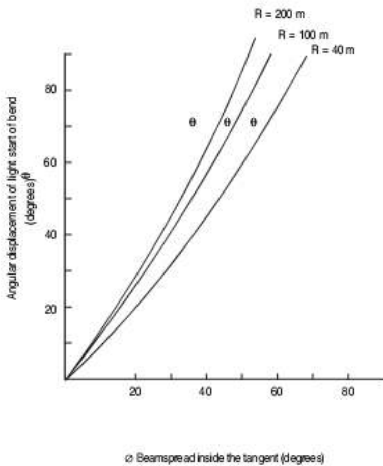
Figure 4-2. Taxiway lighting geometry
